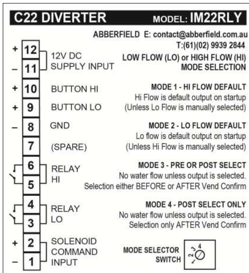
Interface Module IM22RLY Label
