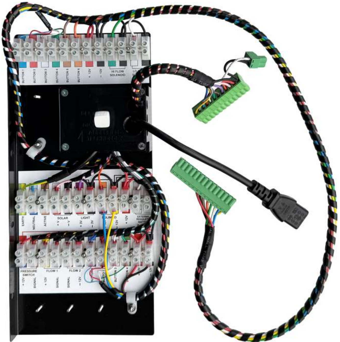
Switch plate with expansion terminal strip as used for Dual Output Control
